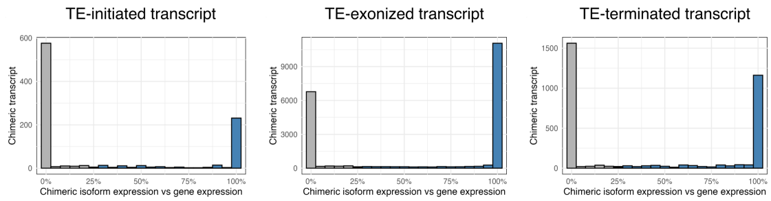
Sup. Figure 8: Histograms with the contribution of chimeric isoform expression relative to total gene expression per chimeric transcript type. Grey bars represent contribution < 25% and blue bars represent contribution > 25%. Chimeric transcripts with contribution < 25% were discarded in this work. TE-exonized transcripts represent the merged result from ChimeraTE: embedded, overlapped and intronic chimeras.
