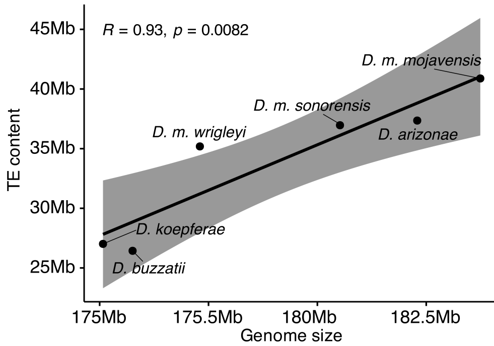
Sup. Figure 2: Correlation between TE content and genome size in the six nanopore genomes of cactophilic Drosophila species.
