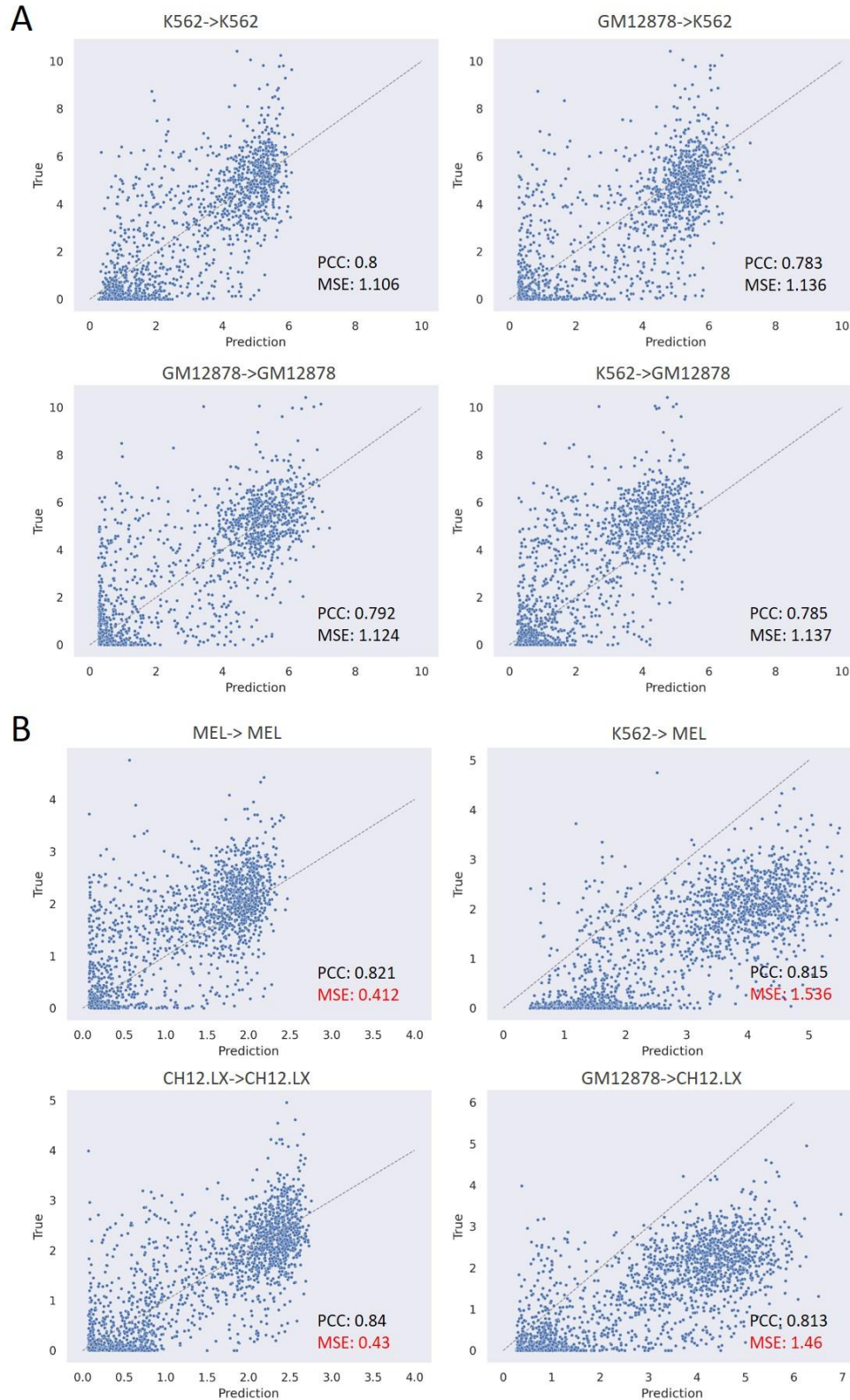
Supplemental Fig S8: Cross-cell type or cross-species predictive performance of ScPGE. (A) The predictive performance of ScPGE when or across cell type, where GM12878->GM12878 indicates using a model trained on GM12878 data to predict GM12878 data while K562->GM12878 indicates using a model trained on K562 data to predict GM12878 data. (B) The predictive performance of ScPGE when or across species, where MEL->MEL indicates using a model trained on MEL data (Mouse) to predict MEL data (Mouse) while K562->MEL indicates using a model trained on K562 data (Human) to predict MEL data (Mouse).
