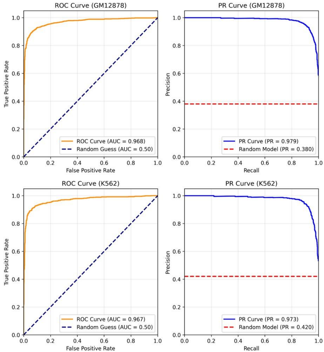
Supplemental Fig S3: The classification performance of ScPGE. The performance was evaluated by the AUC and PRAUC metrics. The random model for AUC was set to 0.5, and the random model for PRAUC was calculated as follows: No. of positive samples / No. of negative samples.
