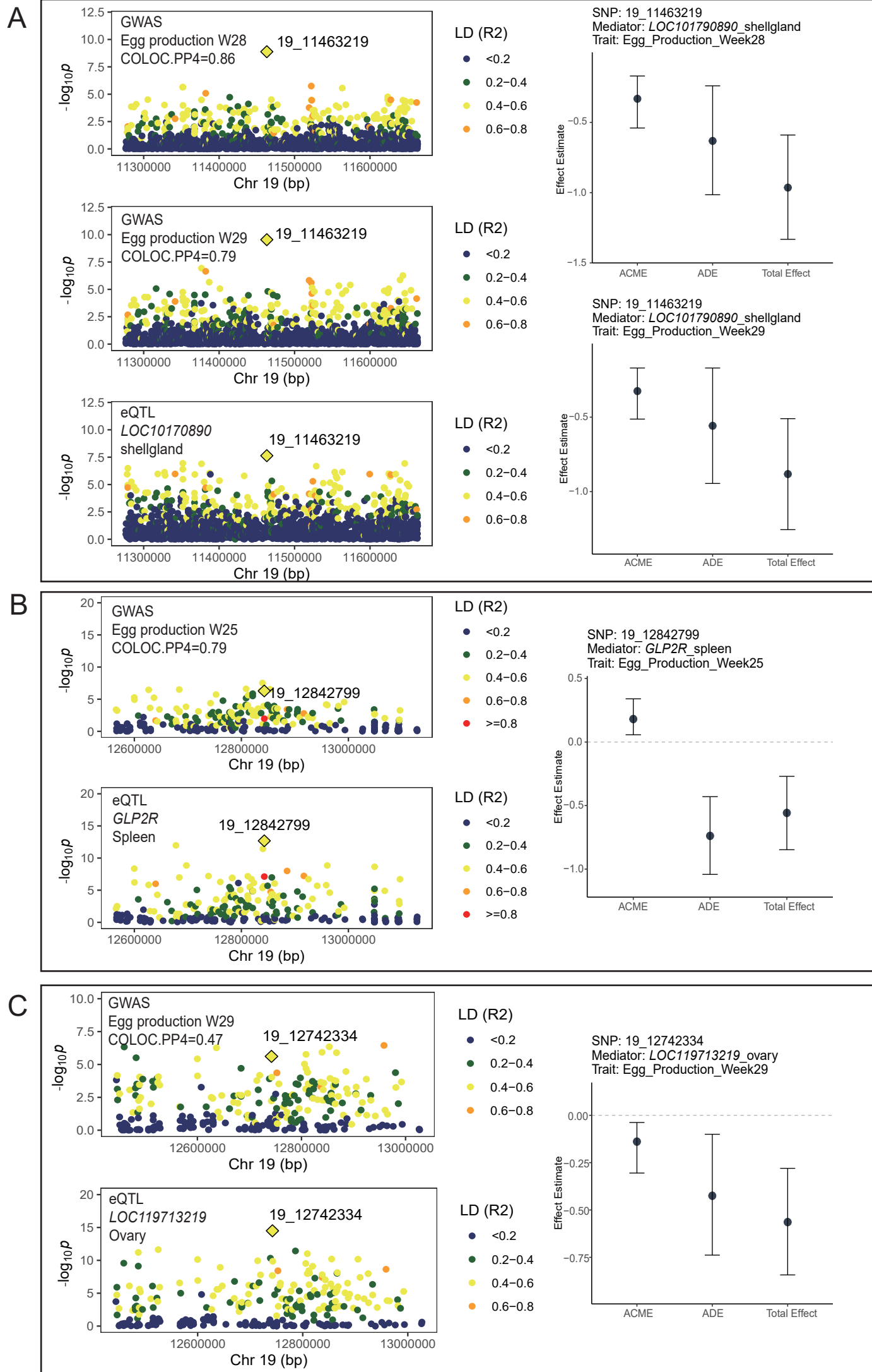
Supplemental Fig S7. The co-localization between molQTL and egg production GWAS.
