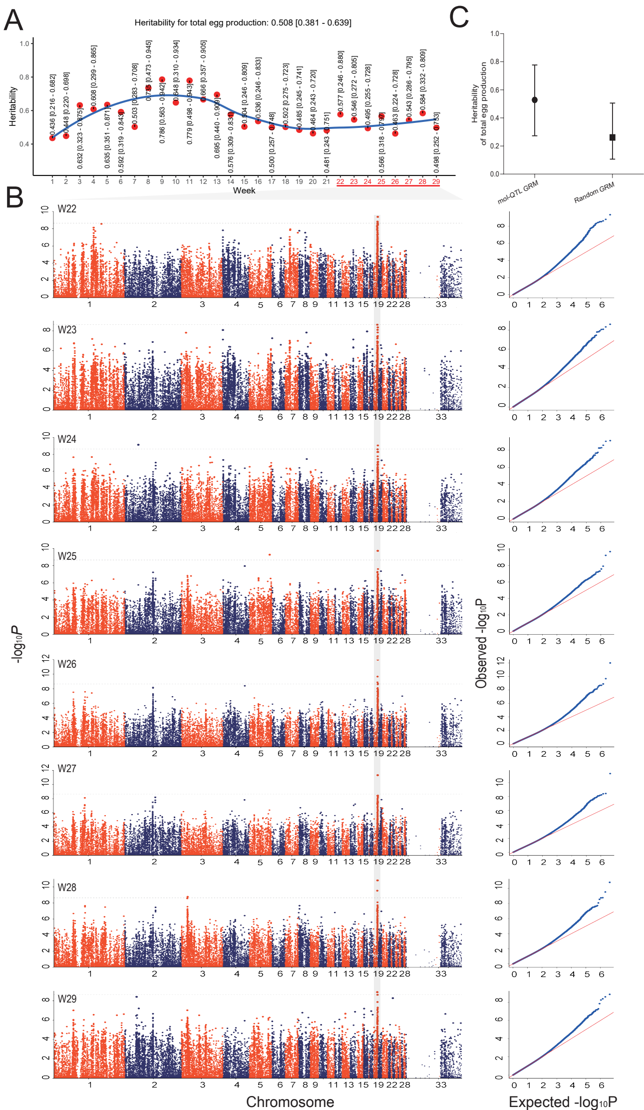
Supplemental Fig S6. The GWAS results of weekly egg production from week 22 to week 29. A. The SNP heritability of each weekly egg production. The values in parentheses represent the 95% confidence intervals. B. The Manhattan (left) and QQ plot (right) for GWAS on the egg production from week 22 to week 29. C. Partitioning of heritability based on SNPs located in the cis-regions of co-localized molecular phenotypes for egg production (molQTL-GRM) and an equal number of randomly selected SNPs (random-GRM).
