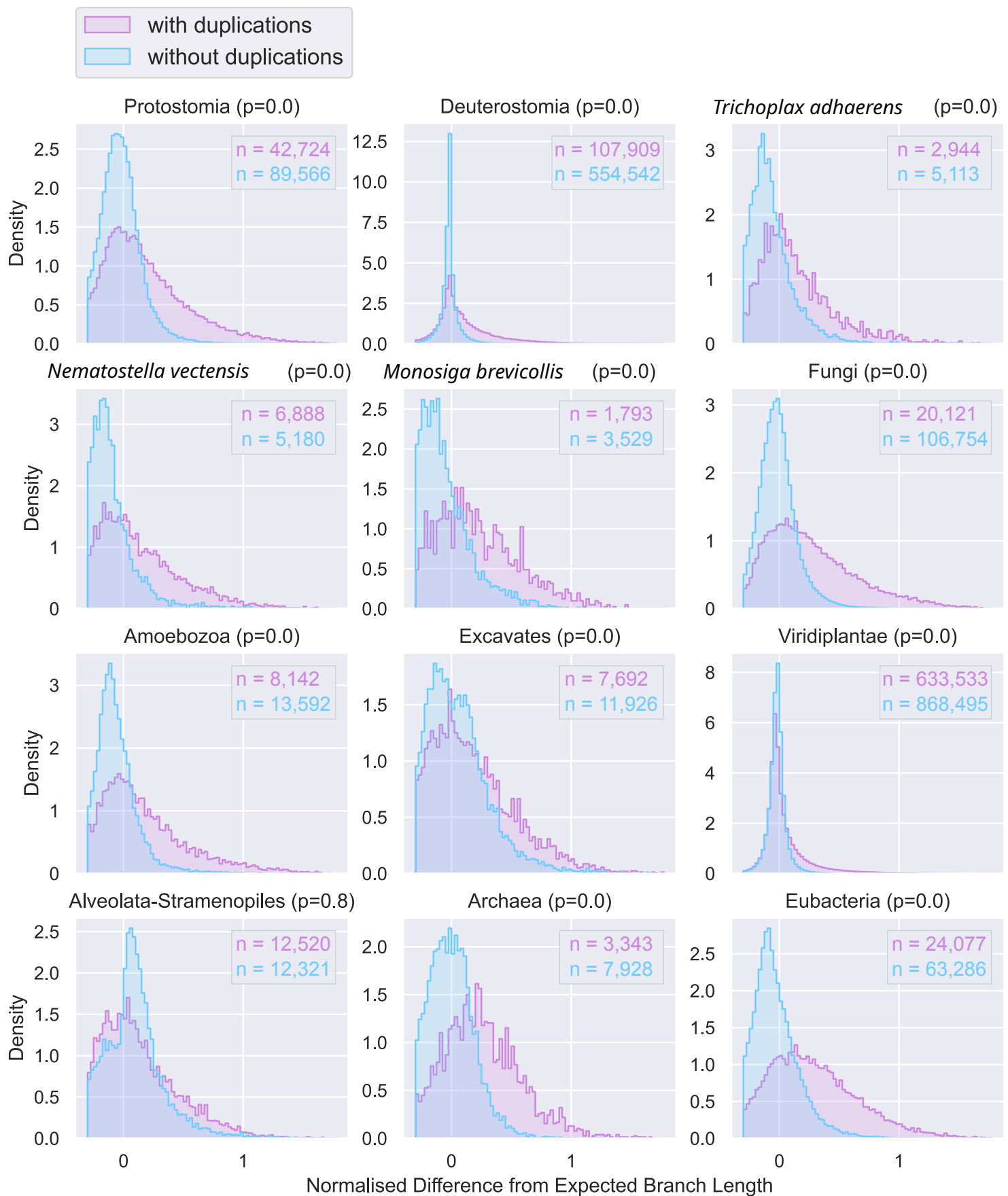
Supplemental Fig. S2. Distributions of the differences between observed gene tree branch lengths and expected branch lengths, with duplications in pink and without duplications in light blue for each major lineage. The p-values for the Mann–Whitney U test are shown in parentheses. The sample sizes (n) are also indicated in each plot.
