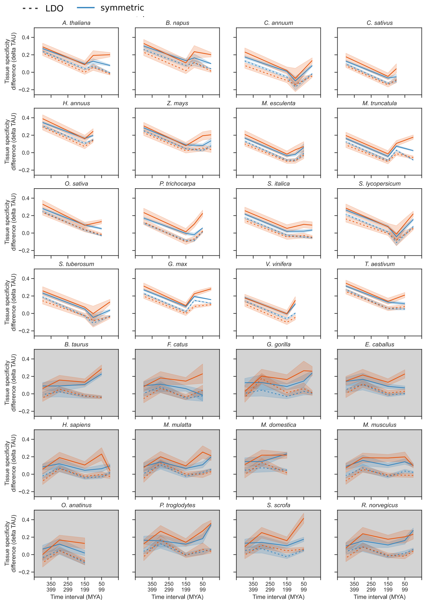
Supplemental Fig. S12. Delta TAU between the closest orthologues and the LDO (dashed lines) and MDO (solid lines) gene following symmetric (blue) and asymmetric (orange) duplications. The x-axis indicates the divergence time between the species compared, in time intervals. Plants are shown on a white background, and animals are presented on a grey background.
