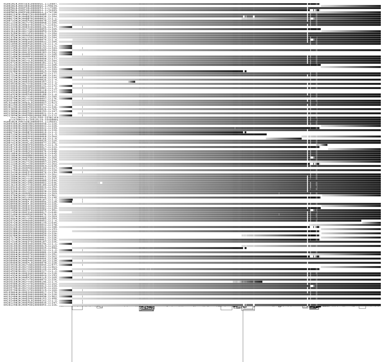
Supplemental Figure S1: odgi visual of the MHC region constructed. One of the plots produced by the odgi viz command by running pggg on the extracted MHC haplotypes of the HPRC assemblies. The plot colors the haplotypes by path position, with the color gradient transitioning from light to dark. Light colors represent the start of the sequence, and dark colors represent the end of the sequence. Many of the haplotypes go from left to right.
