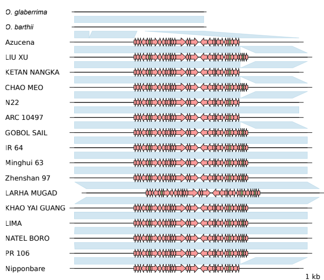
Supplemental Fig. 9 Synteny plot of complex NORGs formed and conserved in O. sativa . Thin lines indicate genomic sequences, red indicates mitochondrial-derived sequences (NUMT), green indicates plastid-derived sequences (NUPT), arrows indicate orientation relative to the mitochondrial or plastid genome, and light blue rectangles between the two genomic sequences indicate regions of collinearity.
