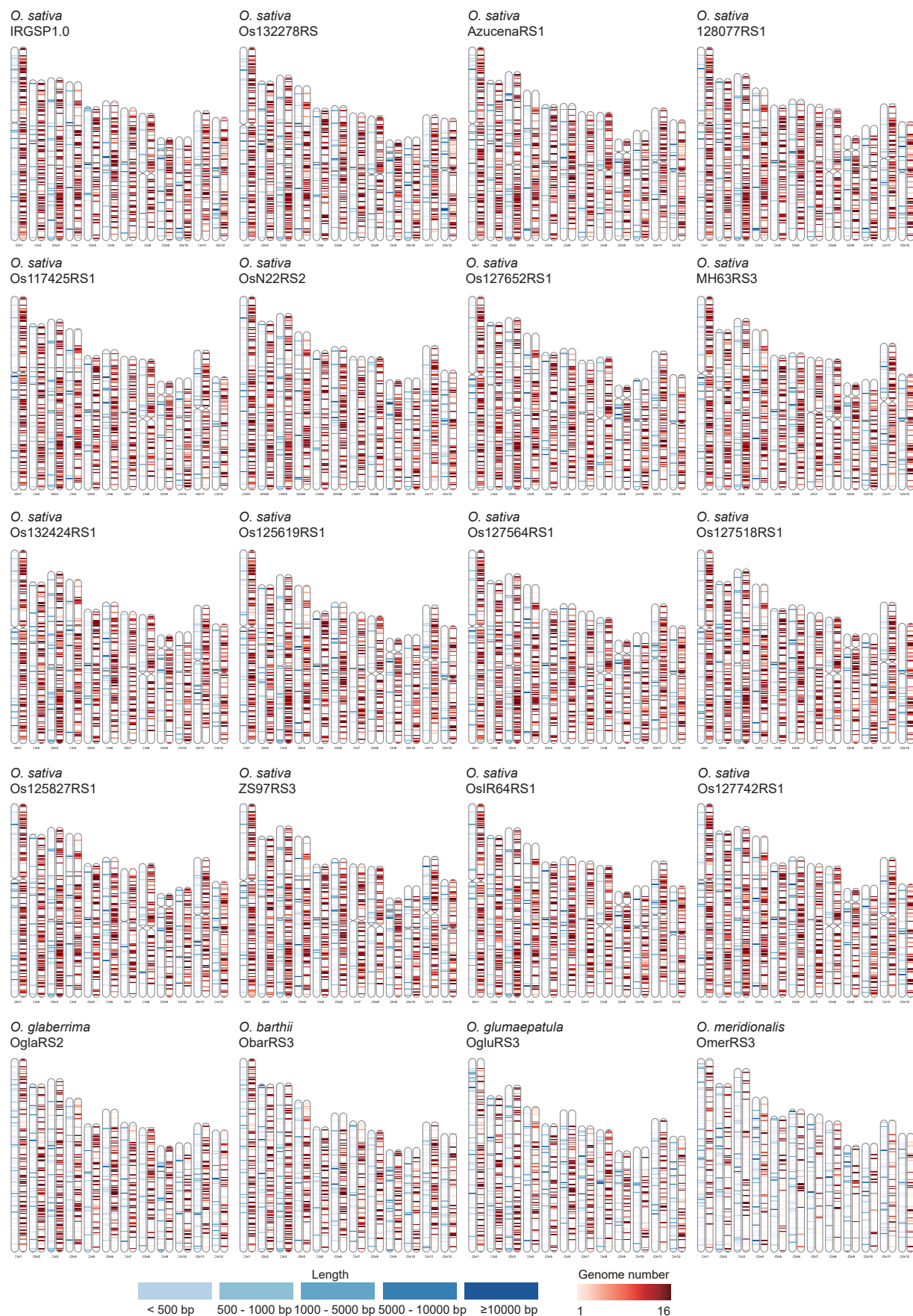
Supplemental Fig. 5 Distribution of ONGs in chromosomes. The NORG length and occurrence frequency in 20 genomes are indicated by different colors.
