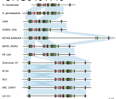
Supplemental Fig. 12 Dynamic changes in NORGs due to TE insertions. Green color indicates nuclear plastid DNA and red color indicates nuclear mitochondrial DNA, arrows indicate orientation relative to the mitochondrial or plastid genome; and light blue rectangles between two genomic sequences indicate regions of collinearity.
