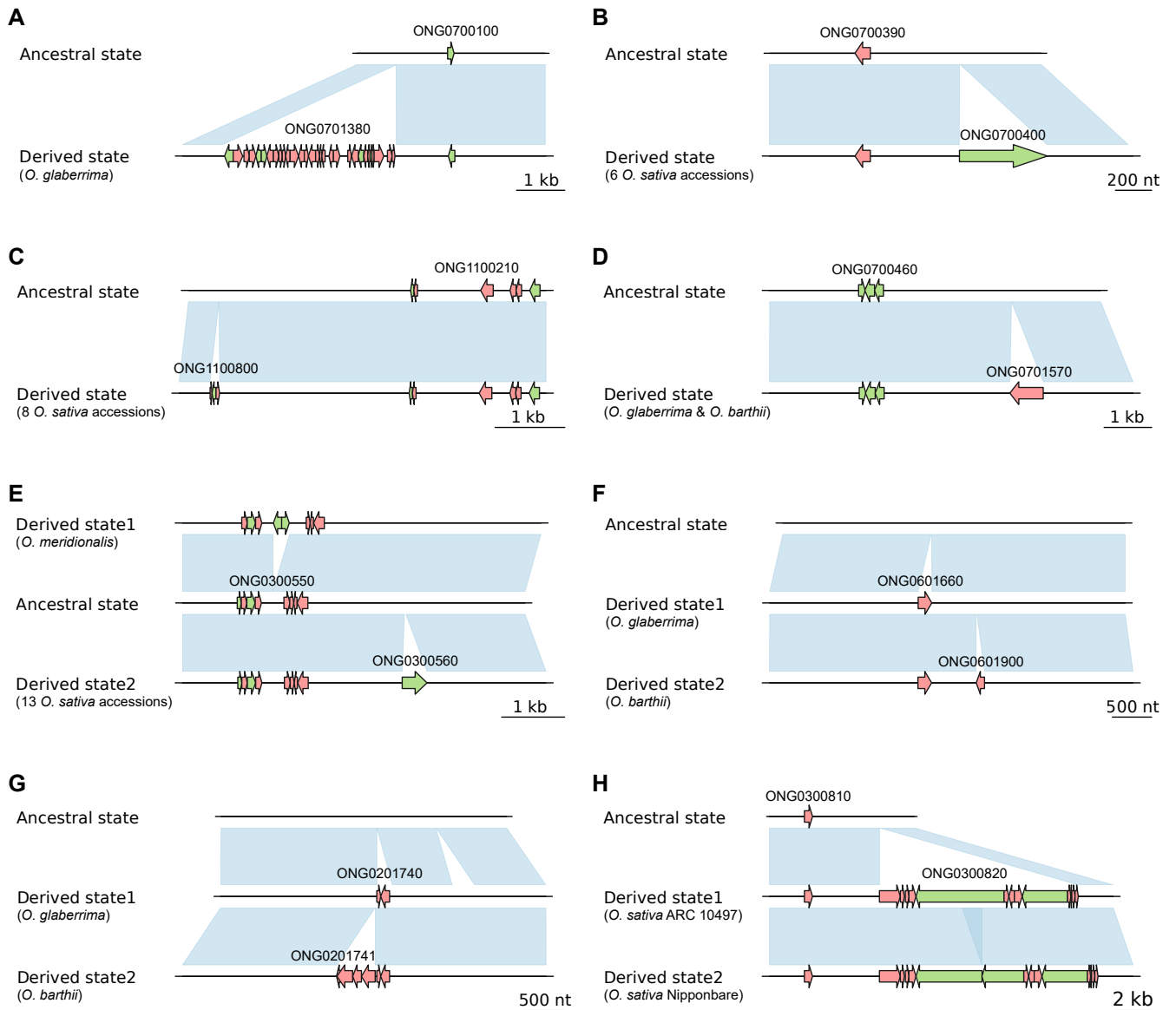
Supplemental Fig. 10. New NORGs inserted near existing NORGs. Thin lines indicate genomic sequences; red indicates mitochondrial-derived sequences (NUMT); green indicates plastid-derived sequences (NUPT); arrows indicate orientation relative to the mitochondrial or plastid genome; and light blue rectangles between two genomic sequences indicate regions of collinearity.
