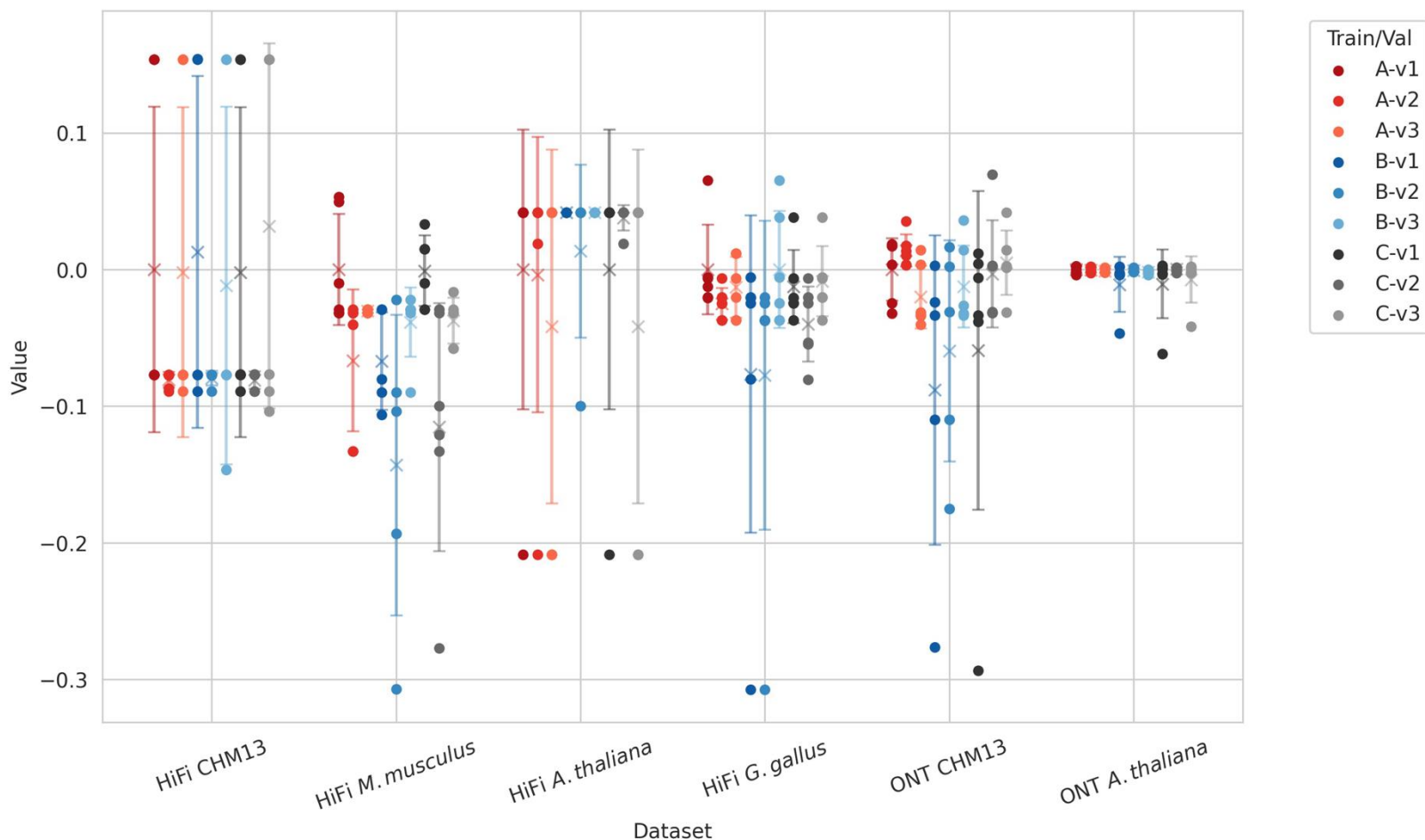
Supplemental Figure S9: Influence of different training datasets on the contiguity of the assemblies. For each choice of training and validation sets, a model was trained six times with six different random seeds. The result of each run is represented with a dot, while the mean is represented with a cross. The error bars show one standard deviation. The value shown is the mean NGA50, normalized to the mean value of the A-v1 training/validation set. Choices A-v1, B-v2, etc. are all described in Supplemental Note S4.
