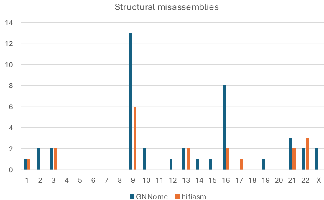
Supplemental Figure S3: Analysis of misassemblies (structural on the left, local on the right) on HiFi CHM13 across chromosomes. Blue bars represent assemblies of GNNome, and orange assemblies of hifiasm.
