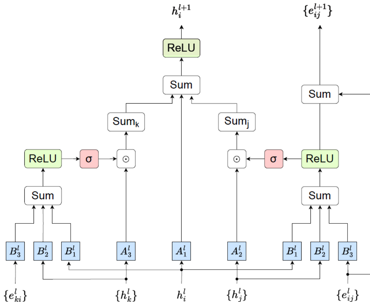
Supplemental Figure S2: Visualization of SymGatedGCN. The arrows show the flow of information.
