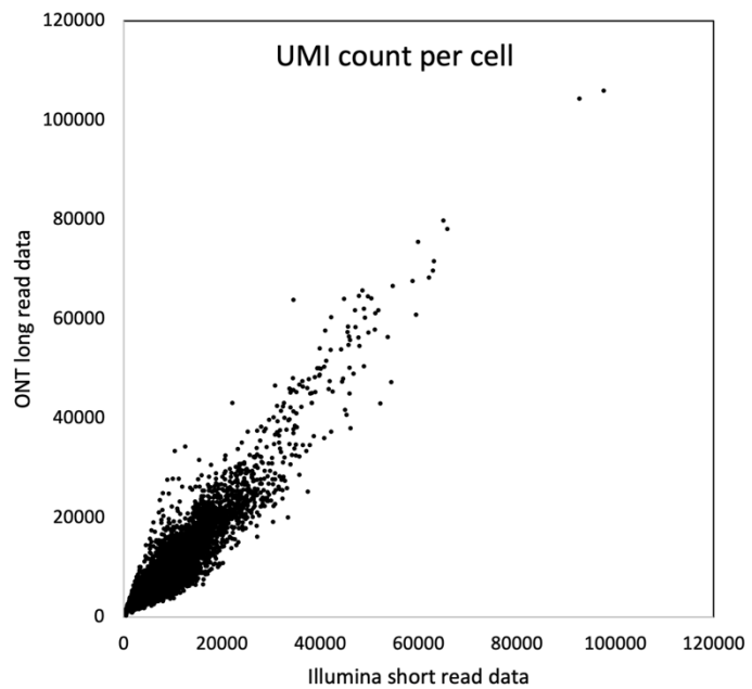
Figure. S3 Comparison of long read and short read data
