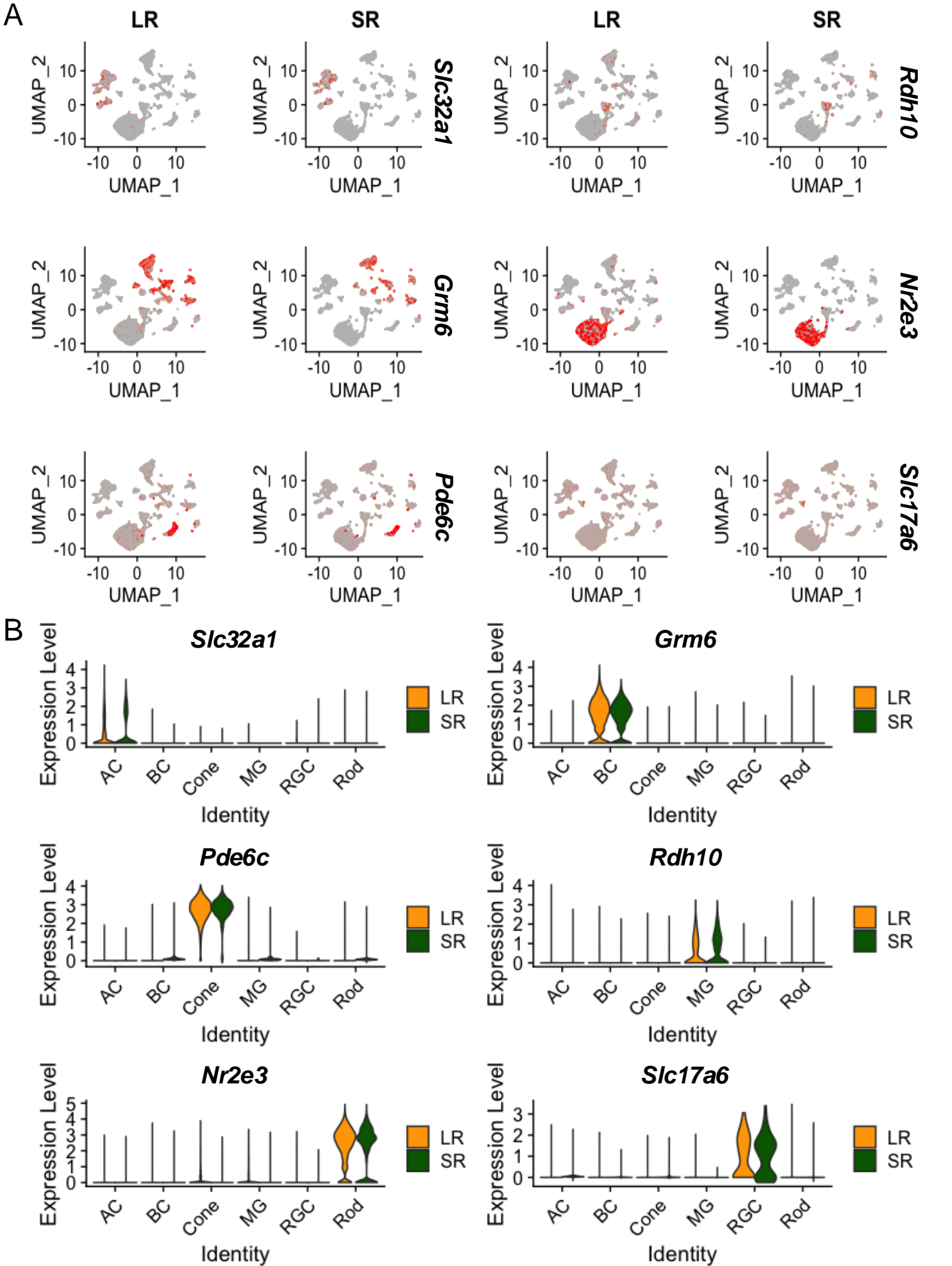
Figure. S2 Comparison between LR and SR at gene level
