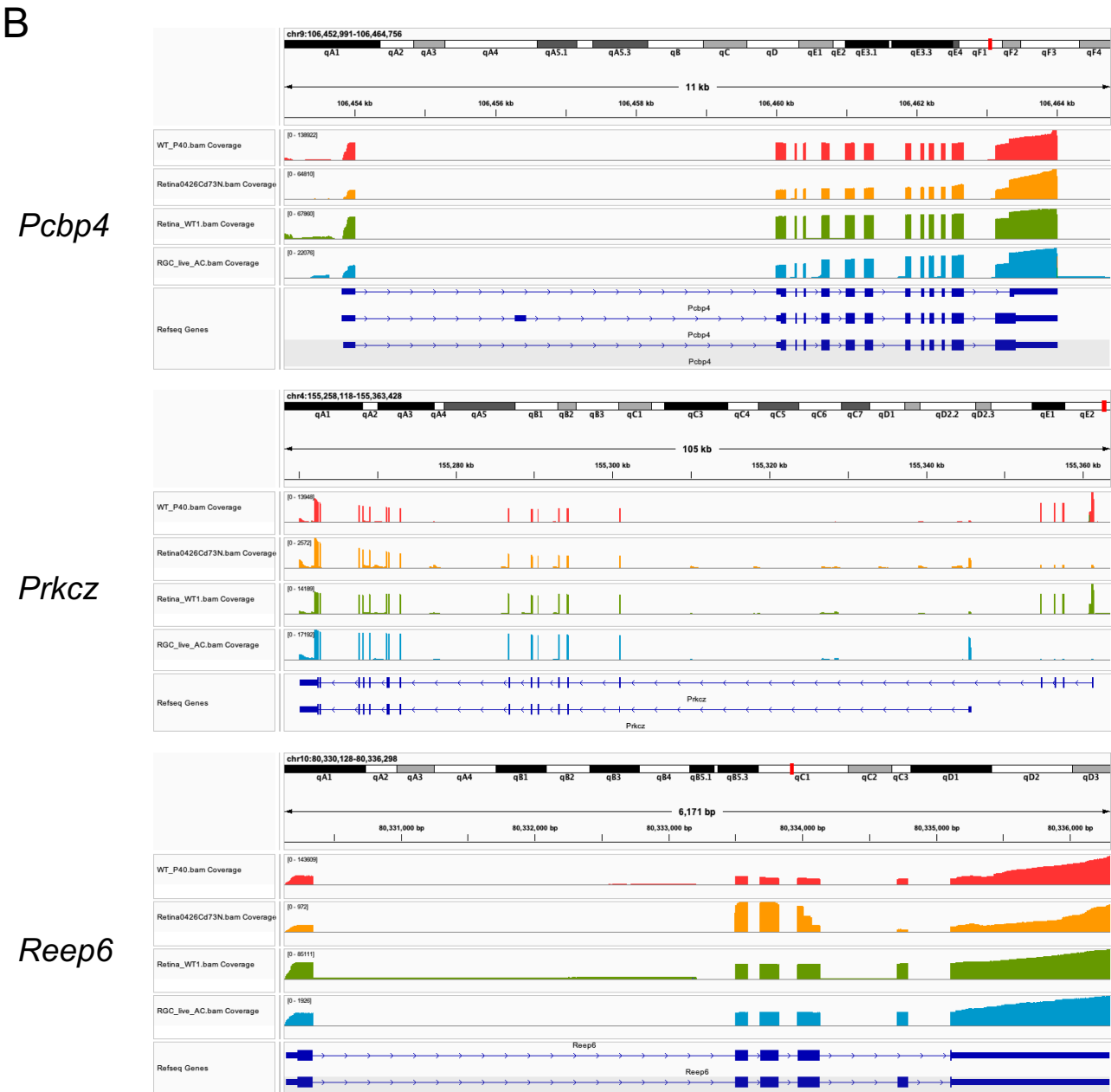
Figure. S1 ONT long read quality
