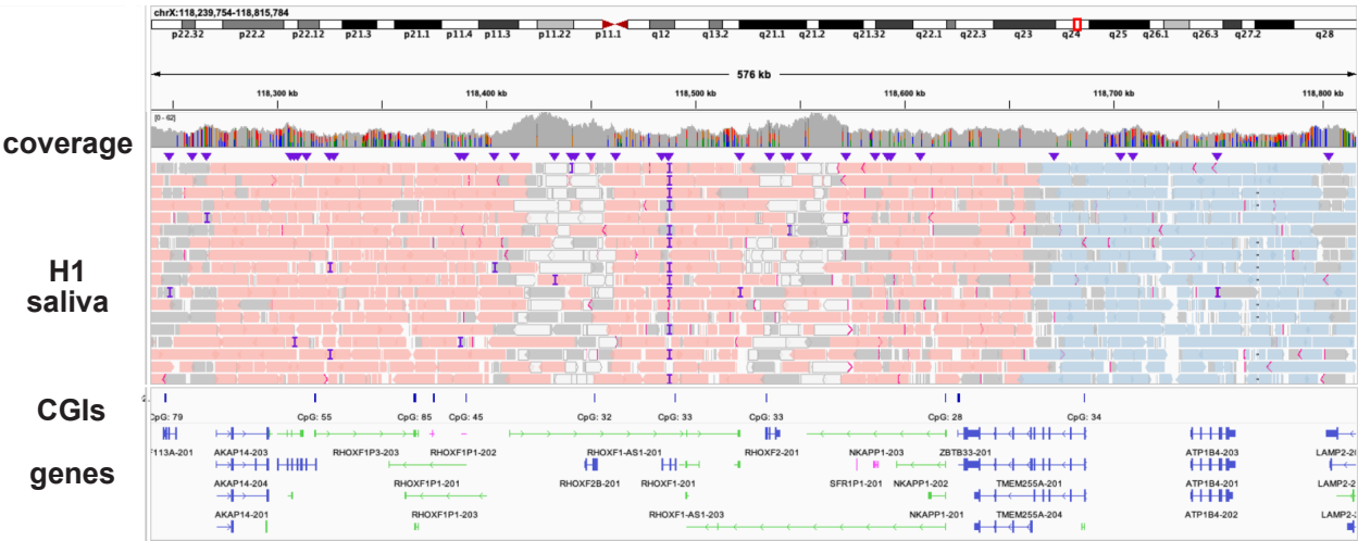
Supplemental Fig. S 1. Skew analysis identifies a phasing error. IGV screenshot of H1 saliva sample reads mapped to the RHOXF2/RHOXF2B region. Reads are coloured by haplotype block. The tandem repeat leads to ambiguous mapping (white reads) and a phase-switching error within the red haplotype block.
