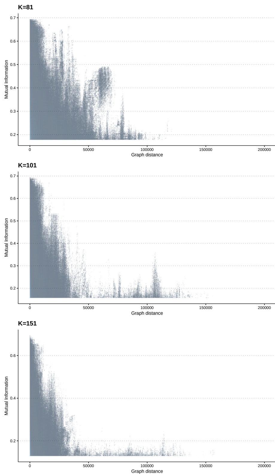
Supplementary Figure 5. Manhattan plots indicating the distribution of MI values by distance with different k -mer lengths in the PAN-GWES pipeline applied to the S. pneumoniae dataset.
