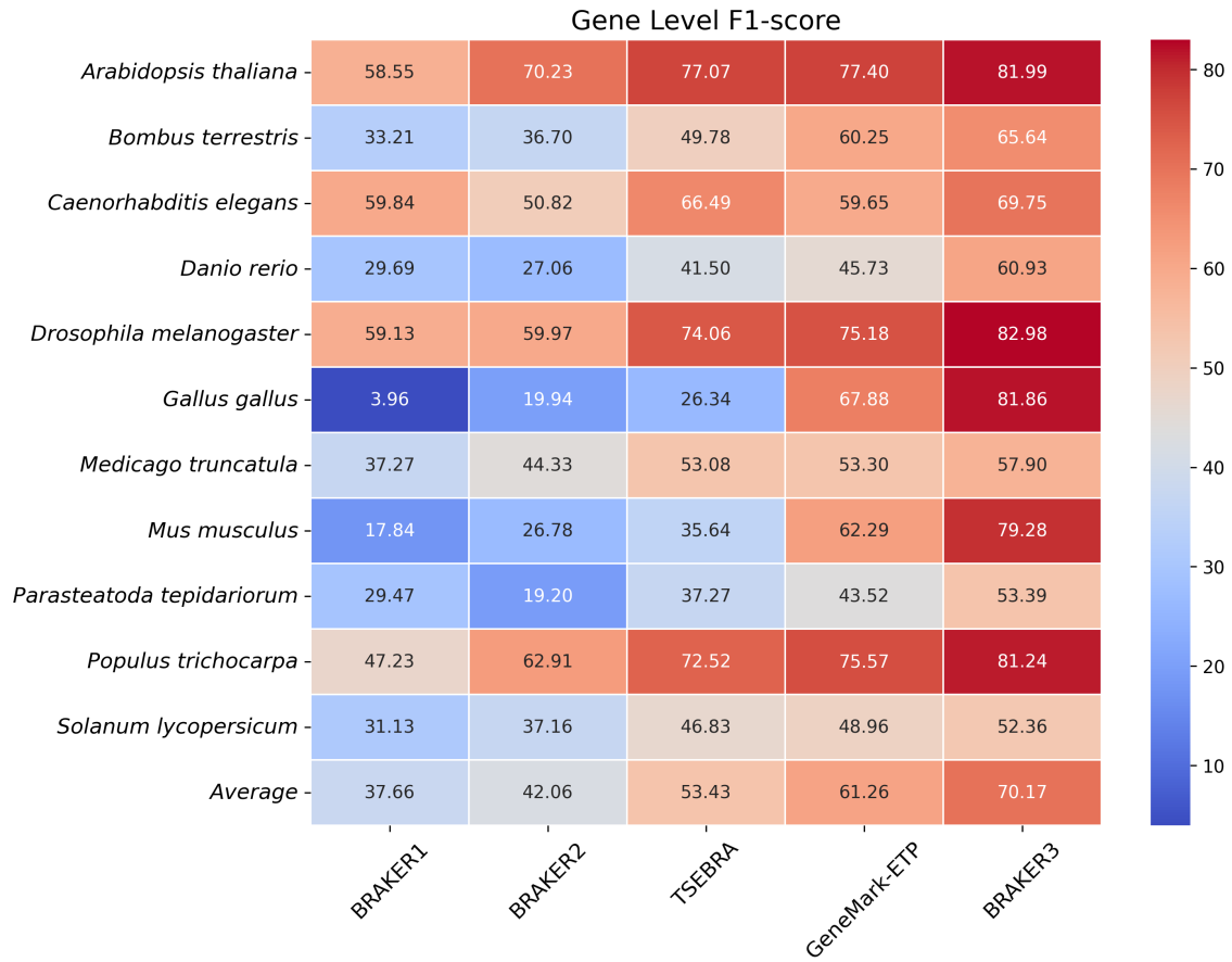
Supplemental Figure S1: Heatmap of F1-scores of pipelines being input short-read RNA-seq libraries and a protein database (with proteins of species from the respective order excluded). The last row shows the averages for the 11 different species.
