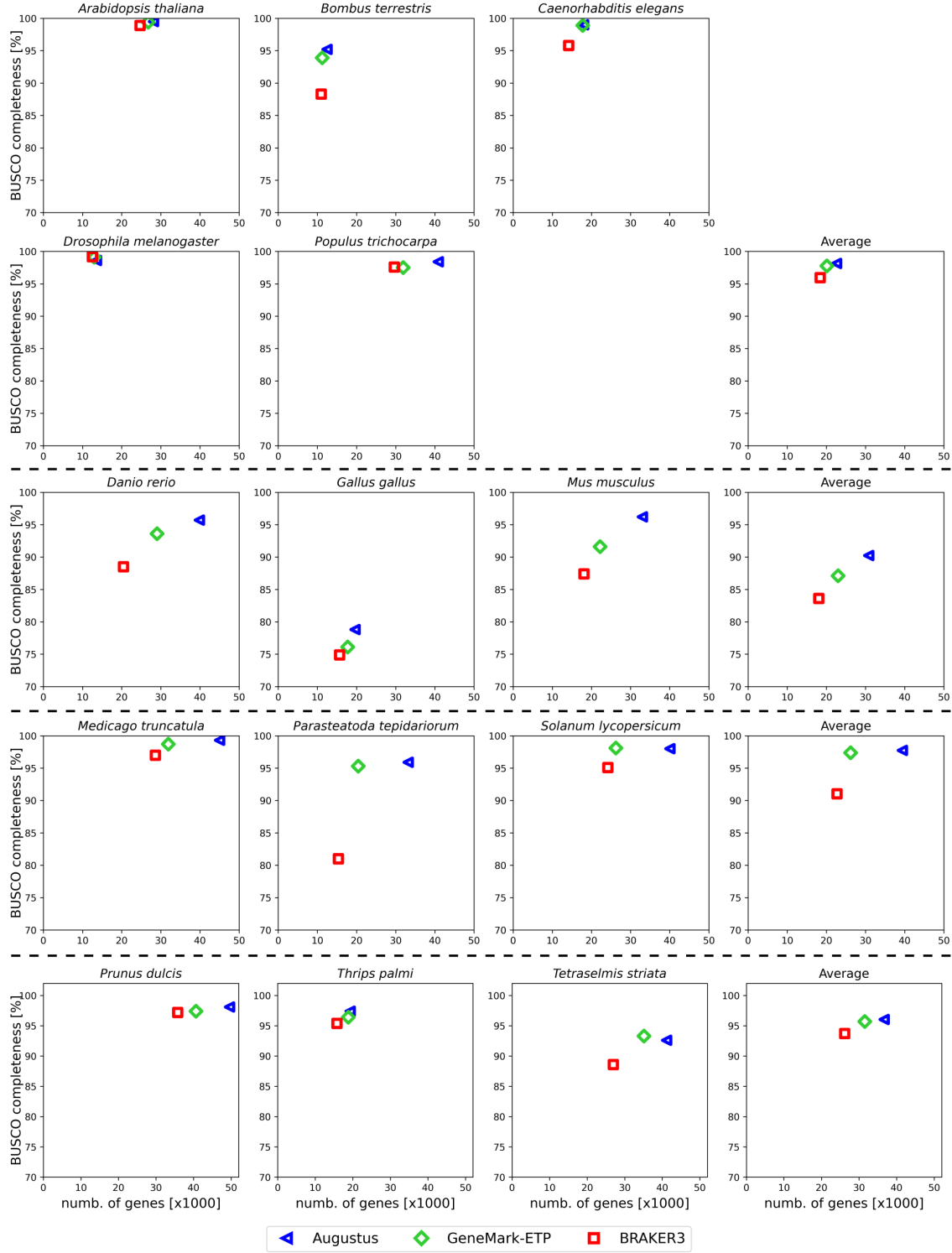
Supplemental Figure S9: Proteome completeness versus the number of genes. The horizontal axis shows the total gene count, after alternative transcripts were grouped into genes. The vertical axis shows the BUSCO completeness percentage (single-copy or duplicated) for the respective gene sets. The AUGUSTUS and GeneMark-ETP gene sets were taken from the output of BRAKER3.
