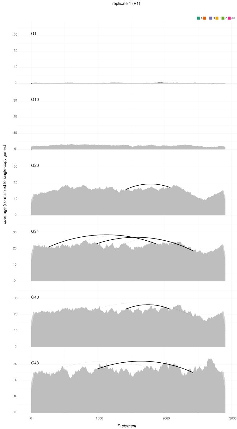
Figure 3: Abundance and diversity of the P-element during the invasion in replicate 1 visualized with DeviaTE Weilguny and Kofler, 2019 . Single-nucleotide polymorphisms (SNPs) and small internal deletions (indels) are shown as colored lines. The absence of colored lines highlights that the P-element has no SNPs or solely SNPs segregating at a very low frequency. Large internal deletions are shown as black arcs.
