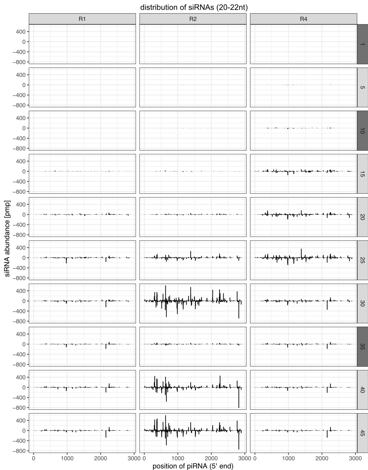
Figure 24: Distribution of siRNAs (20-22nt) along the P-element . Only the 5' positions of siRNAs are shown. The abundance of siRNAs is normalized to one million piRNAs (pmp). Replicates are at the top panel and the generations at the right panel. Sense piRNAs are shown on the positive y-axis and antisense piRNAs on the negative y-axis. We extracted small RNAs either from whole bodies of female flies (light grey panels) or from ovaries (dark grey panels).
