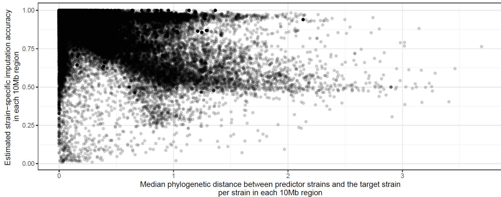
Supplemental Fig. S2. Comparison of median phylogenetic distance of predictor strains to the target strain to strain-specific imputation accuracy. Median phylogenetic distance and strain-specific accuracy was calculated per strain in each 10Mb region across chromosomes 1-19 and X.
