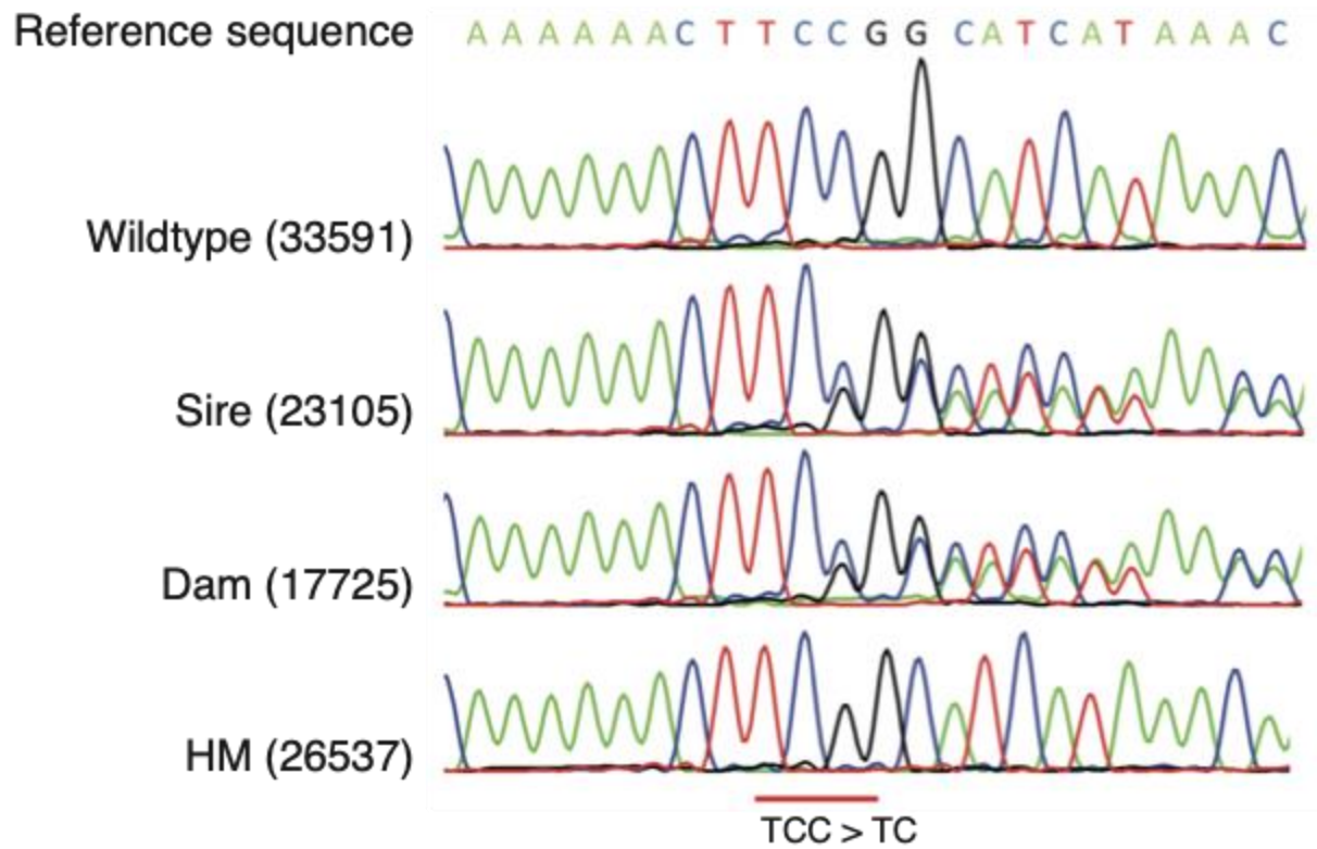
Figure S1. Sanger Validation of mutation. Sanger validation of the frameshift indicates germline inheritance from both parents of 26537. HM= hypermutator. Sire and Dam are parents of 26537.
