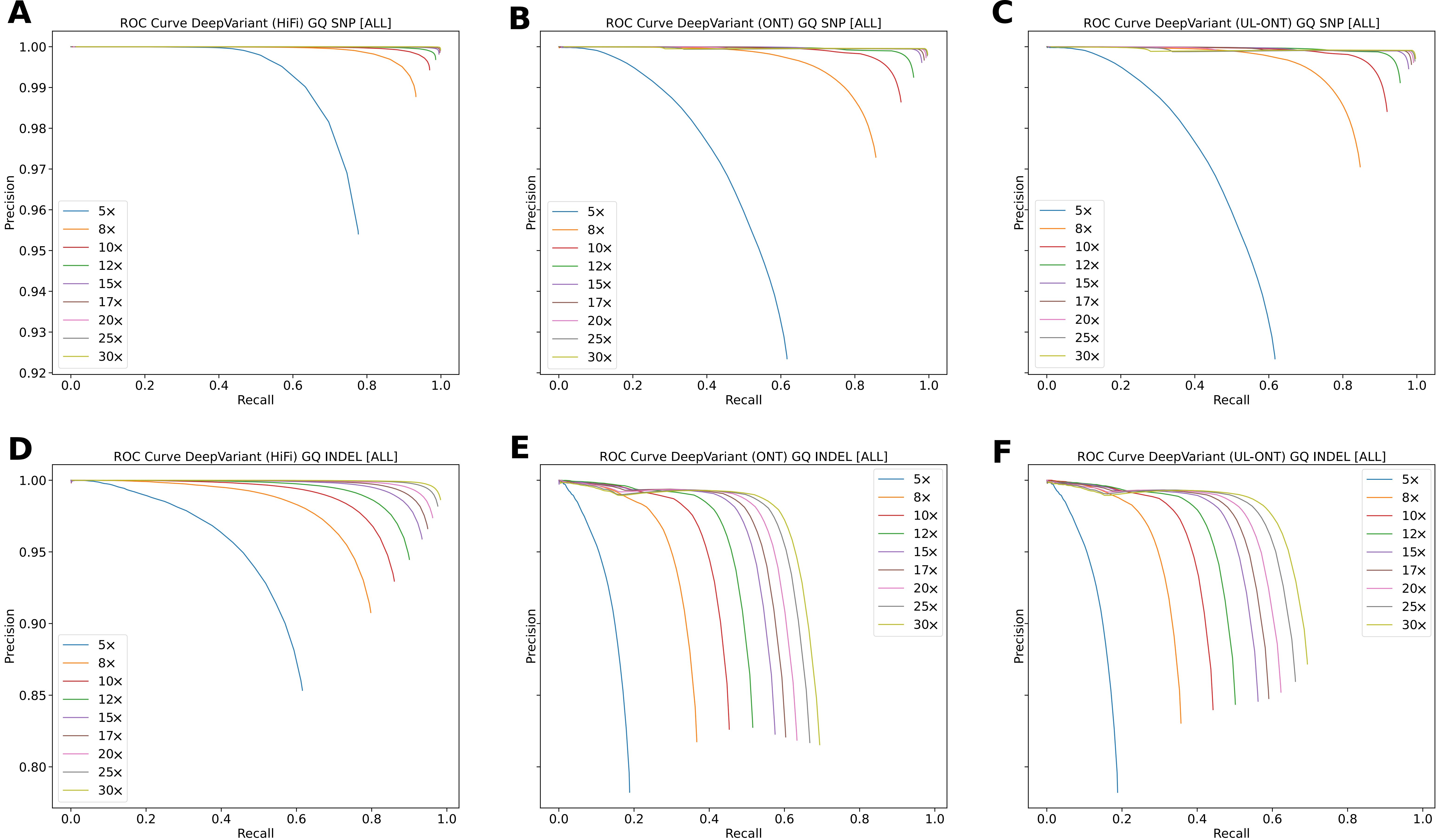
Figure S4. ROC curve analysis as a function of GQ in DeepVariant. ROC curves for DeepVariant SNVs and indels at each of the coverage thresholds for HiFi ( A,D ), ONT ( B,E ), and UL-ONT ( C,F ).
