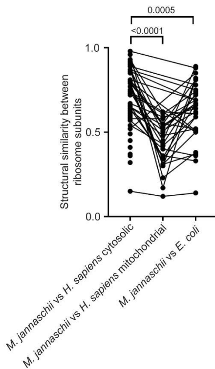
Supplemental Figure S3. Structural similarities between ribosome subunits of M. jannaschii and their annotated orthologs from H. sapiens or E. coli
