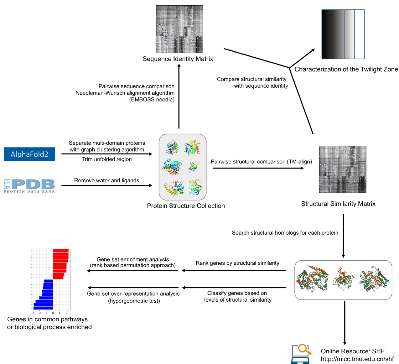
Supplemental Figure S1. Schematic illustration of the workflow and methods used in this study. Pairwise structural alignment was performed with each protein using TM-align. The similarity scores obtained from the alignments were used to portray the distribution of structural similarity and sequence identity, and to evaluate evolutionary conservatives at the protein structure level.
