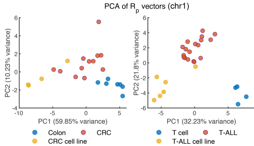
Supplemental Figure S7 Principal component analysis (PCA) for R_p vectors of samples in CRC and T-ALL datasets. The PCA is conducted on R_p values of 40kb bins on Chr1. Each point represents a sample in PC space defined by the first 2 principal components.
