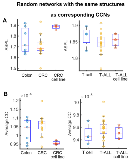
Supplemental Figure S2 Boxplots showing average shortest path length (ASPL) ( A ) and average closeness centralities (CC) ( B ) for random networks of the same number of nodes and edges with corresponding CCNs.
