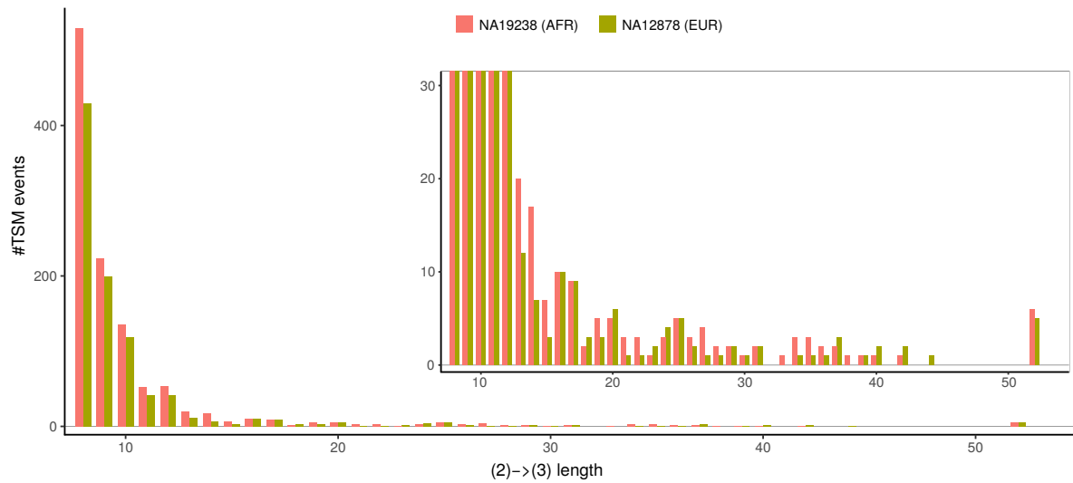
Fig S3. Lengths of inferred TSM events. A great majority of inferred TSM events are 10 bp or shorter in length. Despite the higher numbers of TSM loci identified in African samples, the length distribution of TSM events in individuals of African (NA19238) and European (NA12878) origin are similar. The inset shows lower values. Cases longer than 50 bp are grouped.
