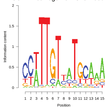
SOX2 motif logo from Sherwood et al.
