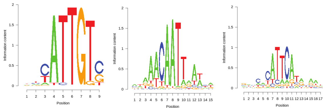
SOX2 motif logo from Sherwood et al.
