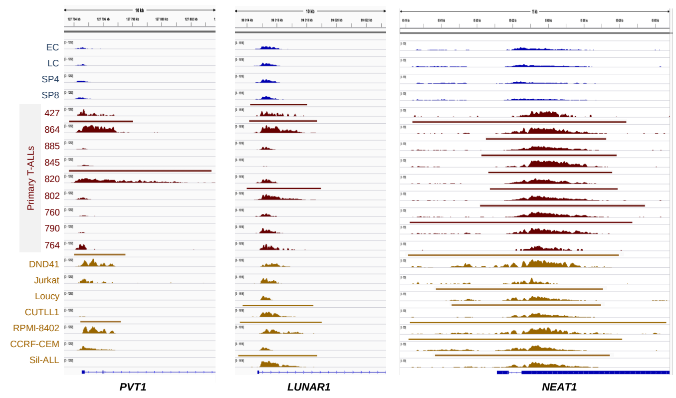
Supplemental Figure S5: Examples of loci associated with broad H3K4me3 domain in T-ALL. Legends are as in Figure 2E.
