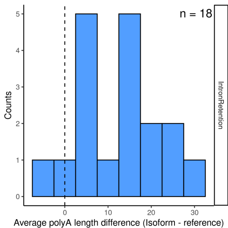
Fig S9. Poly(A) length differences between the isoform and the reference transcript. The plot is for intron retention isoforms with evidence of translation by ribosome profiling data.
