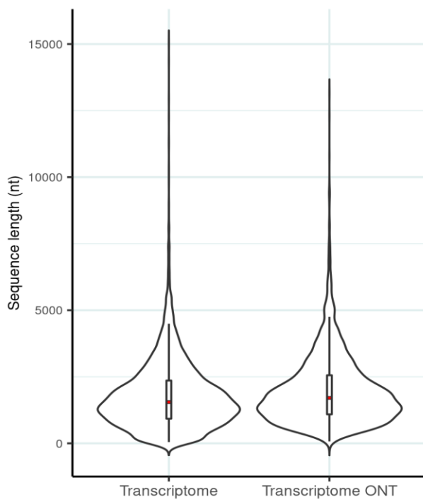
Fig S6. The dRNA-derived transcriptome has a similar length distribution as the known transcriptome. Violin plots of transcript lengths in the Pombase transcriptome (Transcriptome) and the Stringtie transcriptome derived from ONT dRNA reads (Transcriptome ONT).
