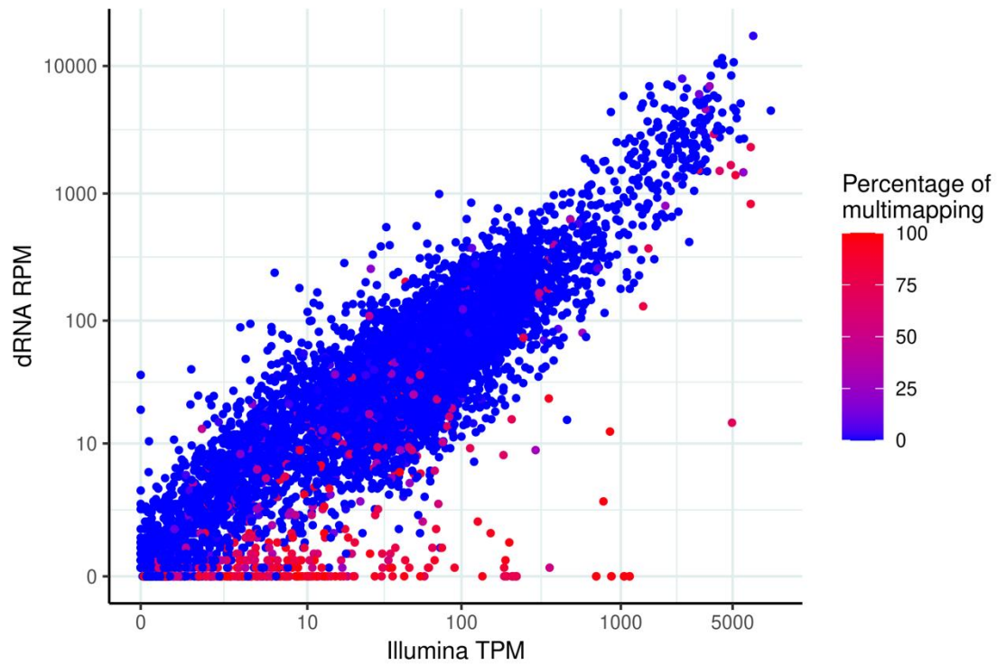
Fig S2. Correlation between transcript abundances with ONT dRNA and Illumina RNA-Seq reads. Transcripts with Illumina multimapping reads were taken into account. The percentage of multimapping is indicated with a color scale. Number of transcripts = 6,799 (expressed in at least one of the two datasets). Expression levels tend to be overestimated in the transcripts with multimapping reads.
