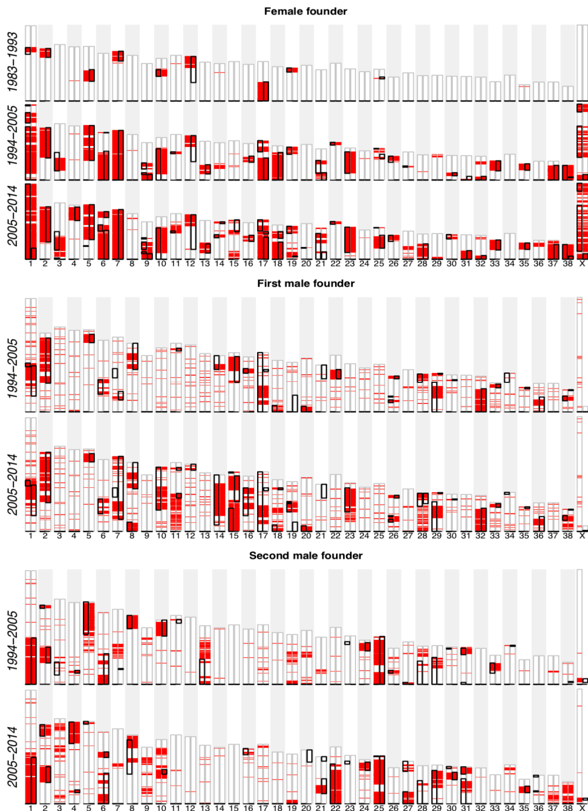
Supplemental Figure S5. Genomic distribution of lost 1 Mb haplotype blocks and individual SNP alleles. Haplotype blocks are displayed as black squares linked to a specific homologous chromosome, while individual SNP alleles are shown as red lines across the two homologous chromosomes. Genomic segments where no lost alleles are displayed within the haplotype blocks are those that are present in several founders, thus allele loss is being masked by other founder haplotypes.
