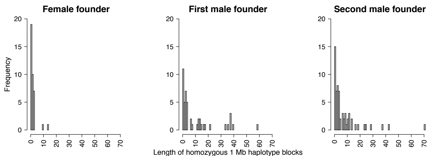
Supplemental Figure S2. Length distribution of the homozygous 1 Mb window blocks observed in three founder individuals of Scandinavian wolf population (x-axes represent the number of adjacent 1 Mb windows in a block).
