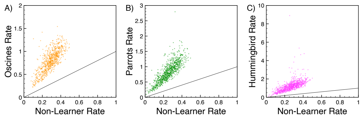
Supplemental Figure S3. Distributions of Acceleration Rates: (A-C) PhyloP estimates for acceleration rate distribution in vocal learners (Oscines A, Parrots B, Hummingbirds C) plotted against the background species vocal non-learner rates, relative to the neutral model estimated from 4-fold degenerate sites by PhyloFit. These can be taken as the average rate for molecular evolution across the group in question at the site. For reference we show a 1:1 line in each figure that would be consistent with the absence of a rate change in the vocal learning lineage.
