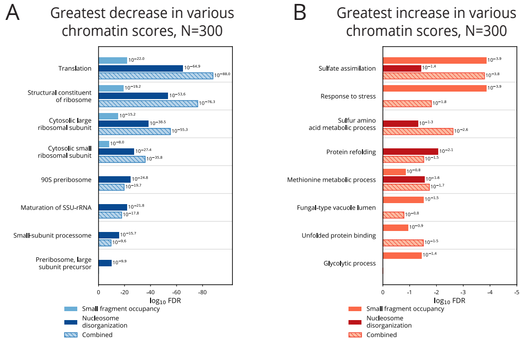
Supplemental Figure S5. GO enrichment analysis of genes with highly dynamic chromatin recovers established cadmium response pathways. (A) Top 8 categories resulting from GO enrichment analysis of 300 genes with greatest decrease in small fragment occupancy, nucleosome disorganization, and combined chromatin score. Translation-related genes are recovered with significant FDR. (B) Top 8 categories resulting from GO enrichment analysis of 300 genes with greatest increase in small fragment occupancy, nucleosome disorganization, and combined chromatin score. Genes involved with stress response, sulfur assimilation, and protein folding pathways are recovered with significant FDR.
