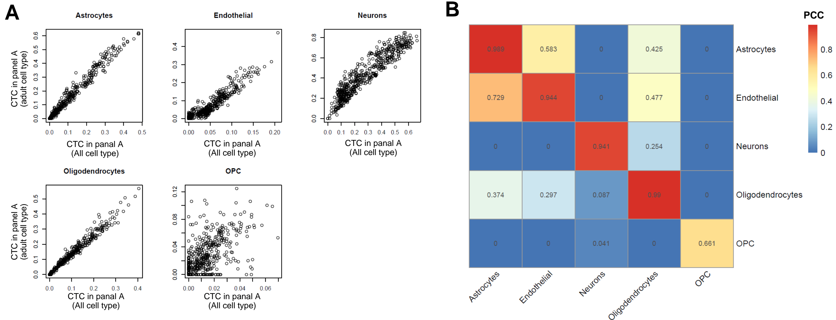
Supplemental Fig. S5. Cell type deconvolution results comparison when using a partially complete reference panel. A , cell type composition (CTC) score comparison. X-axis is the CTC score derived from both adult and fetal reference panel (all 17 cell types from panel A), y-axis is the CTC score derived from adult reference panel (6 cell types, including astrocytes, microglia, neurons, oligodendrocytes, oligodendrocyte precursor cells (OPC), endothelial cells). B , Pearson correlation coefficient of different cell type CTC score when using different cell type reference. Only cell types with an average CTC score > 0.01 were compared.
