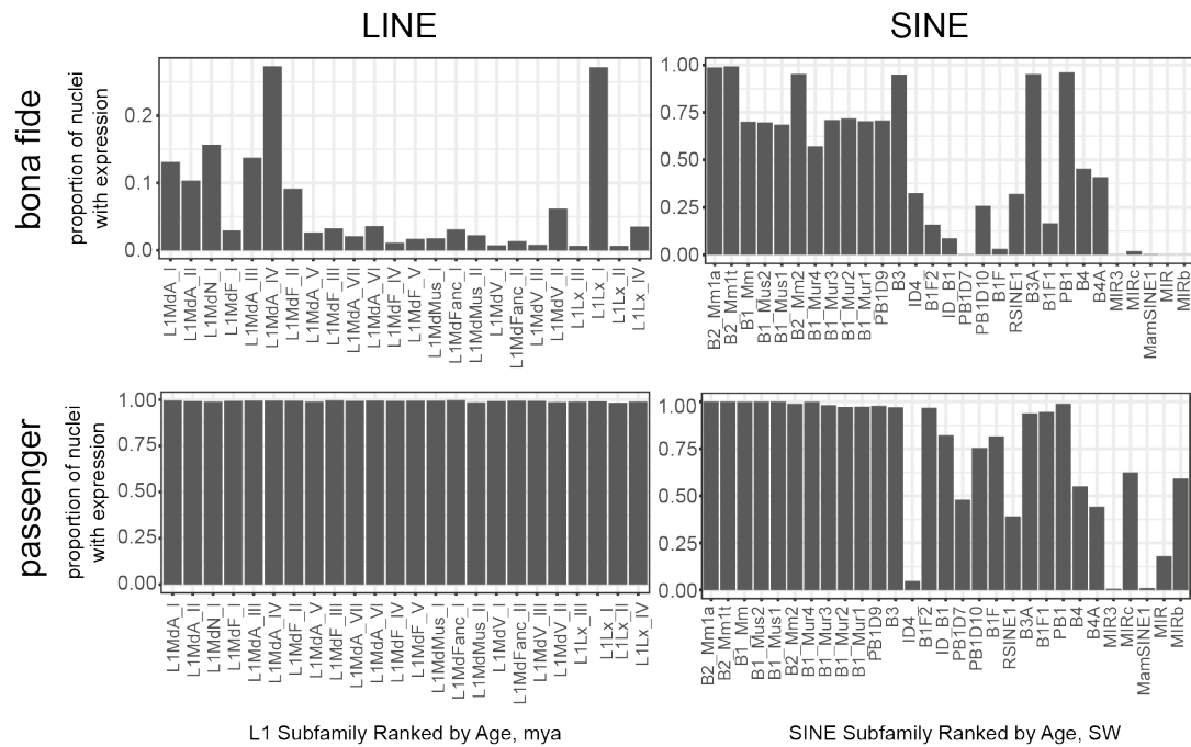
Supplemental Figure 1. Distribution of LINE and SINE element expression
