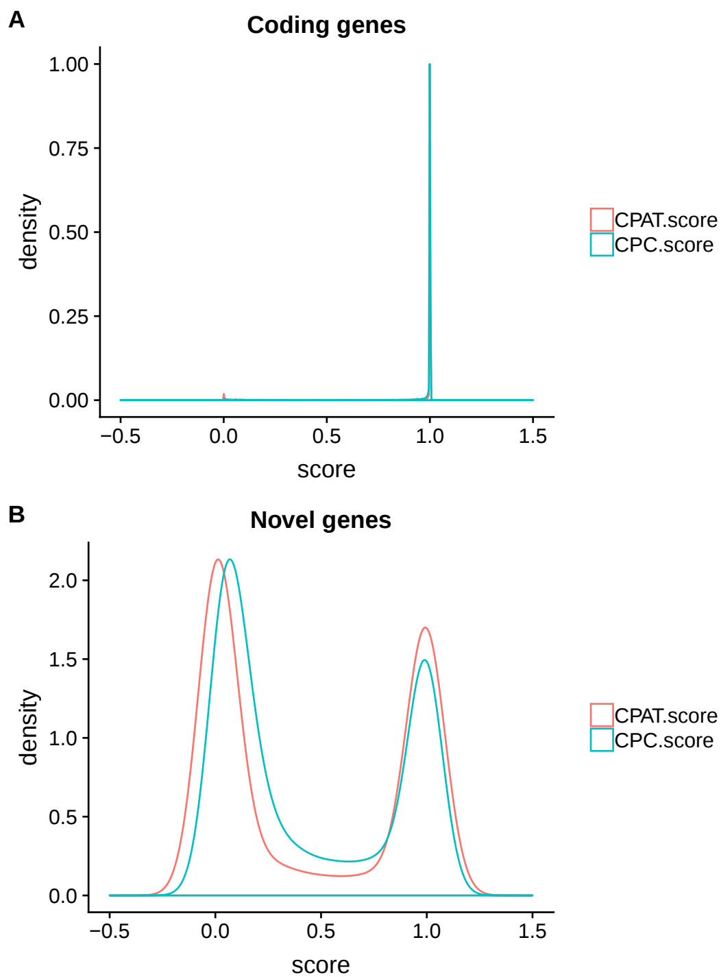
Supplementary Figures 5: Coding potential scores of coding genes and novel genes calculated by CPAT and CPC.
