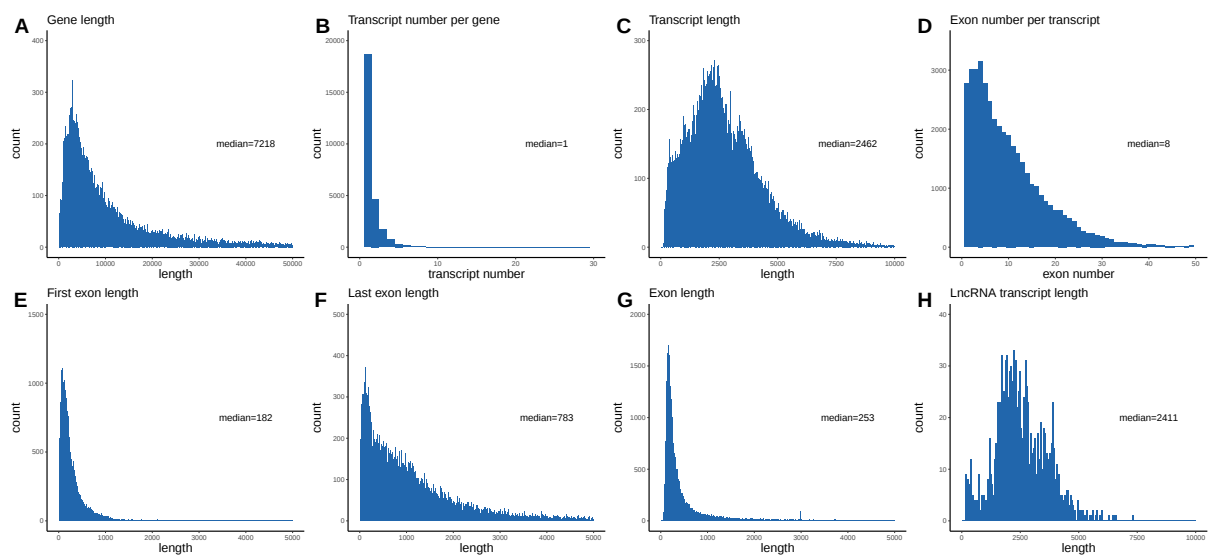
Supplementary Figures 3: Characteristics of IGDB models. (A-H) Distributions of gene length, number of transcripts per gene, transcript length, number of exons per transcript, first exon length, last exon length, exon length, lncRNA transcript length.
