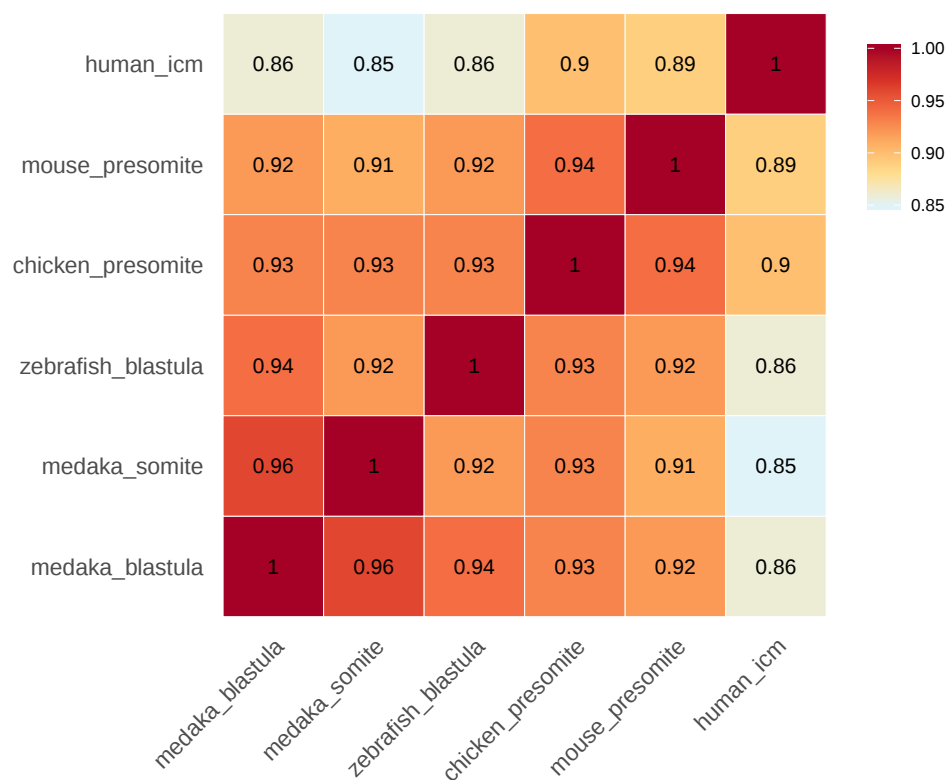
Supplementary Figures 20: Pioneer scores of medaka blastula (stage 11) , medaka somite (stage 19), zebrafish blastula (dome), chicken presomite (HH6), mouse presomite (E7.5) and human ICM are highly correlated.
