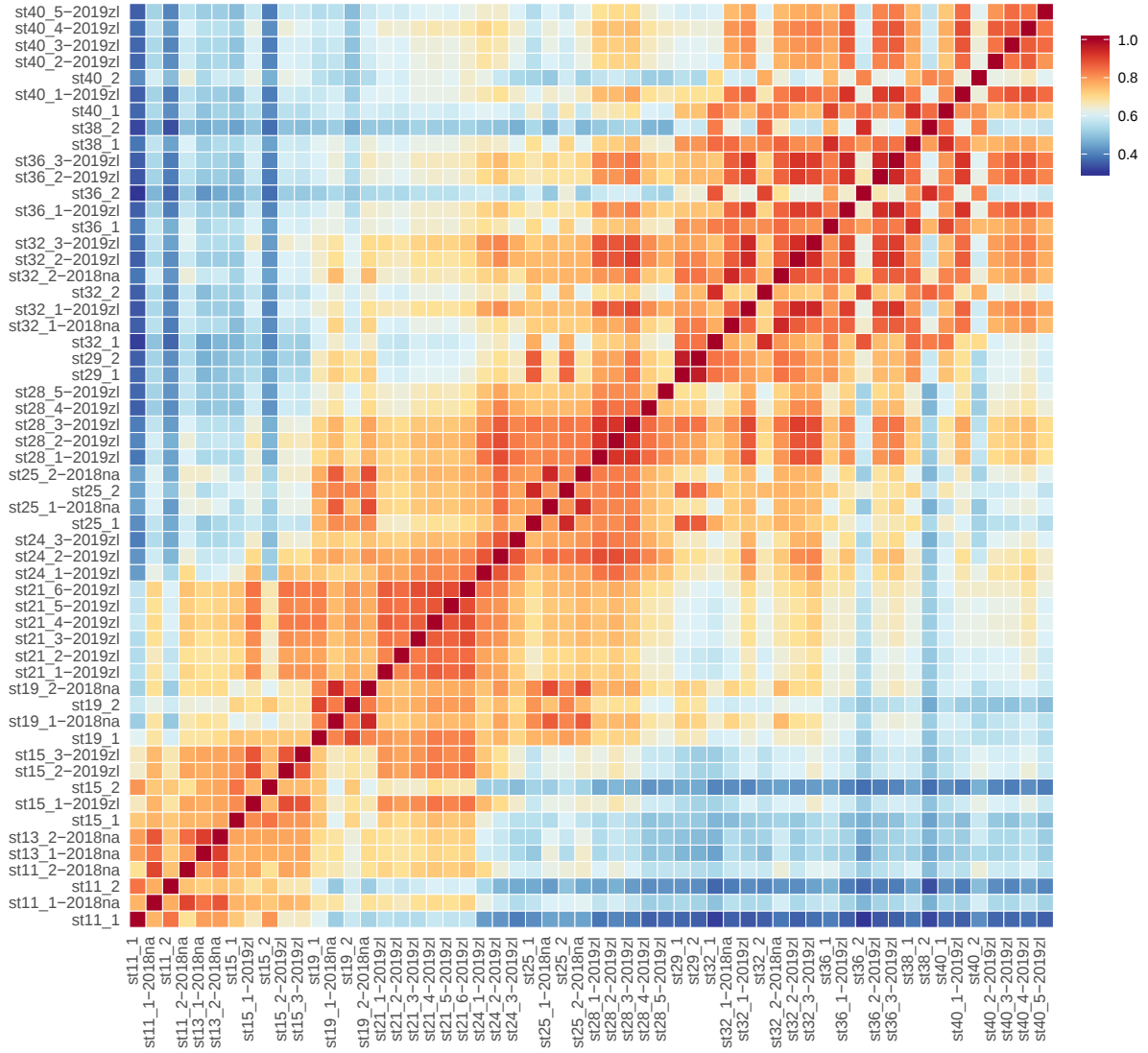
Supplementary Figures 14: Spearman's correlation among our ATAC-seq data and previously published data. All public samples are denoted by '2018na' or '2019zl'.
