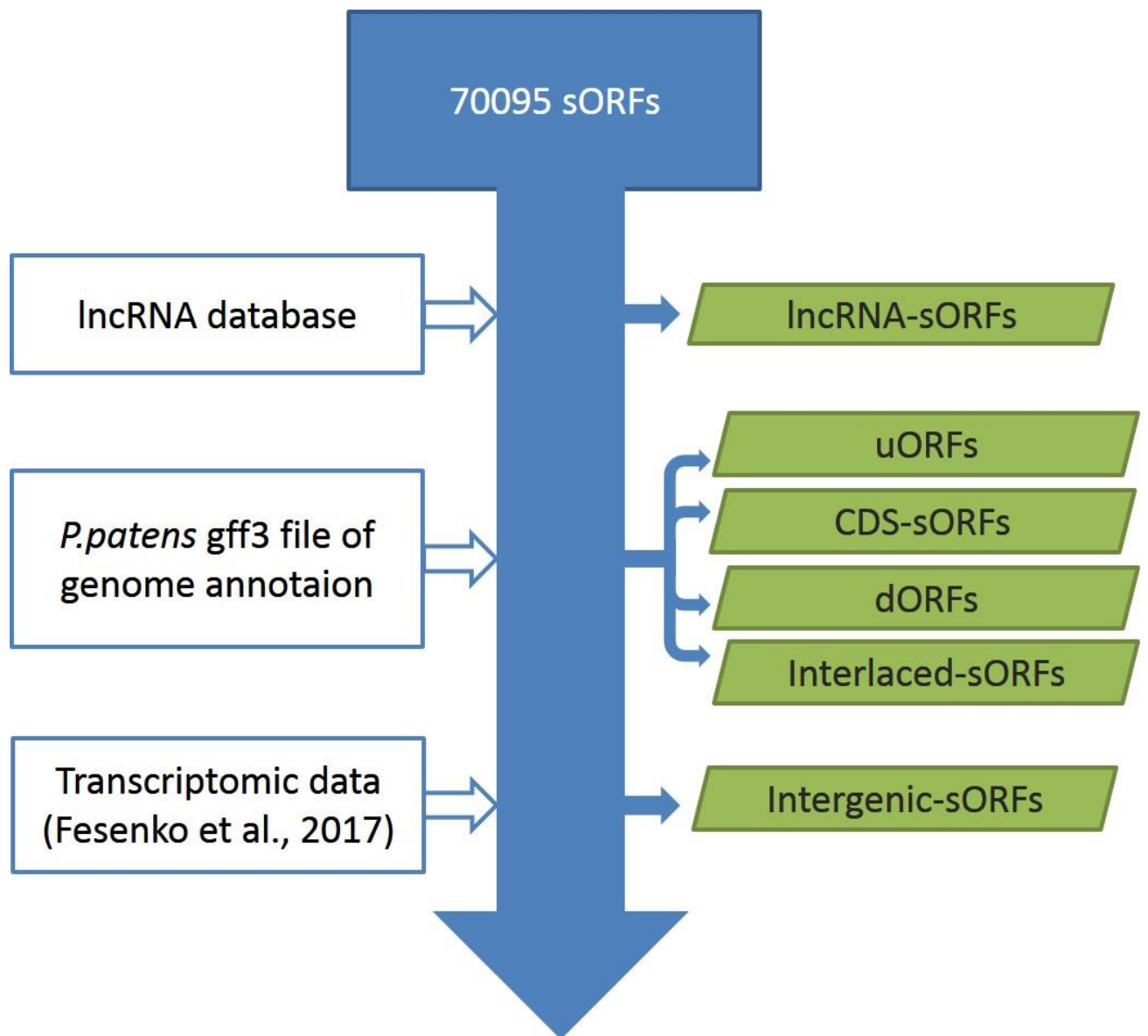
Supplemental Fig. S17. sORF classification procedure used in this study.
