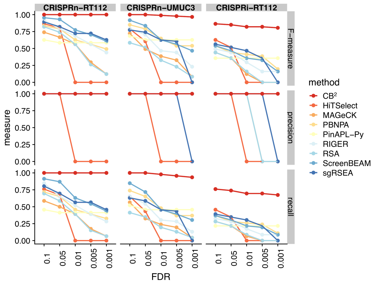
Supplemental Figure 7. CB 2 outperformed all other methods in F1, precision and recall measures on Evers et al. (2016)'s screen data. F1-score (top), precision (middle) and recall (bottom) for each method on three benchmark datasets are presented as a function of FDR cut-off values.
