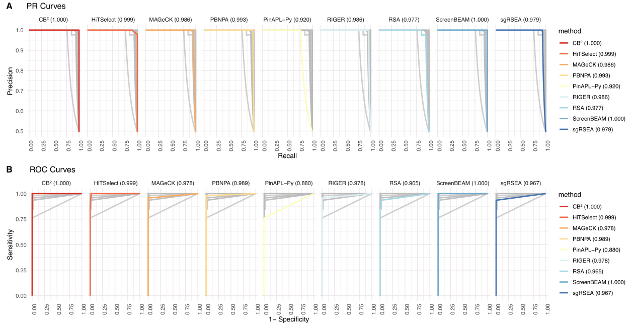
Supplemental Figure 4. Precision-Recall (PR) curve and Receiver operating characteristic (ROC) curve comparison of different methods using CRISPRn-RT112 dataset from (Evers et al. 2016). (A) PR curves for each method. A bracket-surrounded number right to a name of the method indicates area under the curve (AUC) of the corresponded PR curve of the method. (B) ROC curves for each method. A bracket-surrounded number right to a name of the method indicates AUC of the corresponded PR curve of the method.
